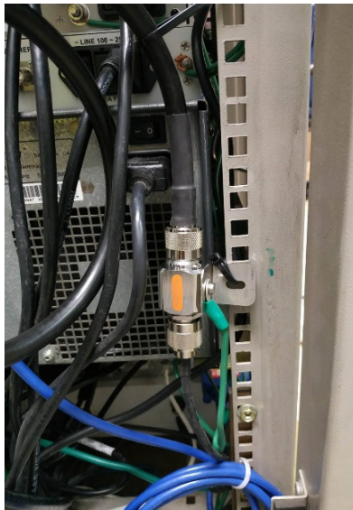
-Lightning arrester for NTP GPS, NTP GPS Network Time Server, Training
